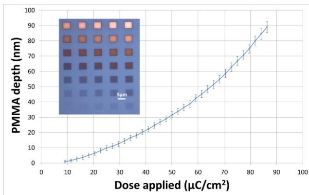
Figure 1. PMMA depth after e-beam exposure and pure MIBK development as a function of the exposure dose. Measurements were made on the sample shown in the embedded image exhibiting different colors corresponding to different topographical levels of the resist. Matrix is composed of 5 \times 5 \mu\text{m}^2 squares and dose is increasing from left to right and from bottom to top.
