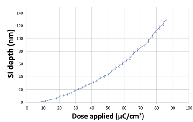
Figure 2. Si mold depth after transfert by ICP-RIE using previous grey-scaled PMMA as a mask
