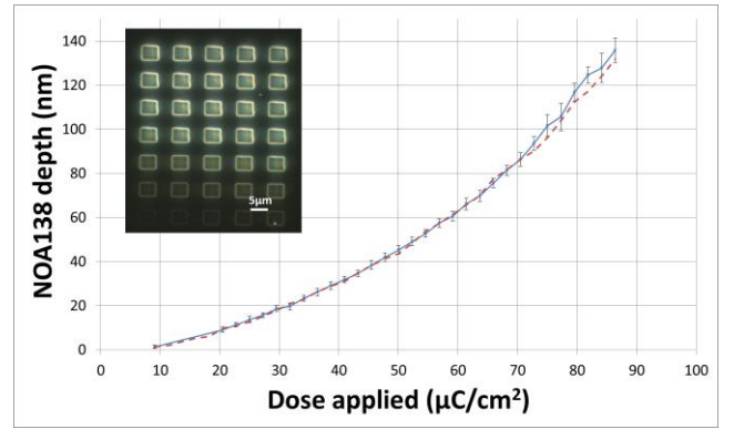
Figure 3. NOA138 depth after UV-NIL on bulk Si as a function of the exposure dose. Measurements were made on the sample shown in the embedded image made in darkfield optical microscopy due to the poor contrast between NOA138 and the substrate in brightfield illumination. Border brightness of each square increases with the resist height in each square corresponding to different topographical levels. Dashed line represent the silicon mold depth as it can be seen in Figure 2 for comparison.
