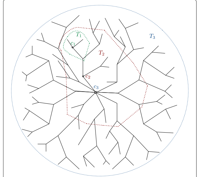
Fig. 2 Optimal graph convergence on a tree. In every round, robots compute a sequence of trees ordered by containment
