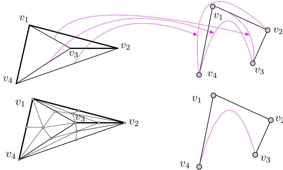
Fig. 6 Topological perspective of graph convergence. Top Solving a tree by three processes. Bottom Trying to solve a tree in one round
