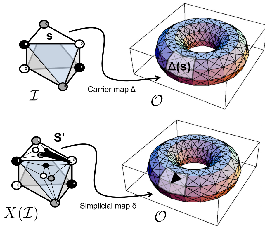
Fig. 8 The wait-free computability theorem. A graphical description of the wait-free computability theorem
