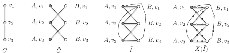
Fig. 7 Topological perspective of edge-covering. G and colored graph \tilde{G} , with input \tilde{I} and views after one round X(\tilde{I}) , for robots A, B
