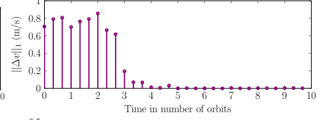
Fig. 12: Impulses and convergence from X_{04} for controller C.
