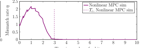
Fig. 15: Impulses and convergence from X_{04} for the MPC controller.
