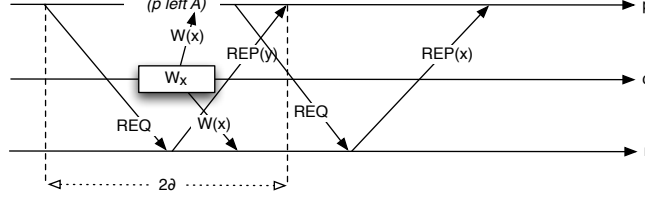
Fig. 3. Example of race condition for REP(y) messages
