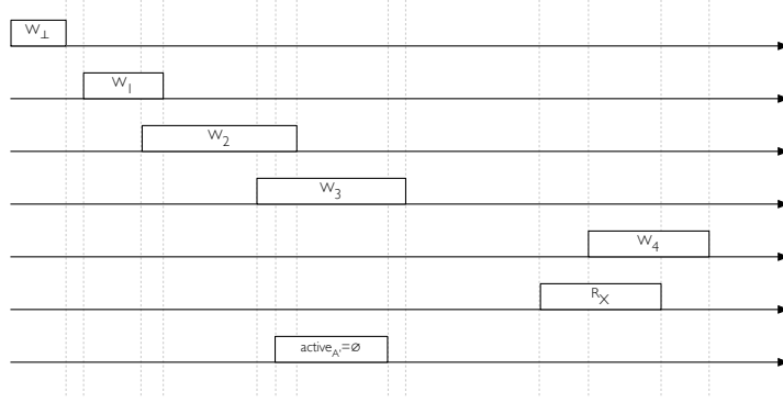
Fig. 5. An execution scenario with concurrent writes from distinct processes.
