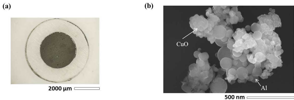
Figure 1: (a) Picture of one Al/CuO nanothermites pellet (Al/CuO nanopowders compacted into a Nylon washer) and, (b) SEM picture ( \times 150\,000 ) of Al/CuO mixture before compaction and prepared at an equivalence ratio of 1.2.
