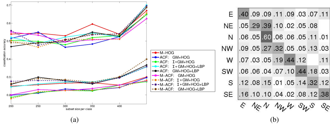
Figure 7: (a) The classification accuracy for upper bodies have been evaluated considering the exact precision, acc1 (lower curves), and the adjacent orientations, acc2 (upper curves), has been plotted as a function of the amount of samples for each class; the extreme data points correspond to using the whole training set. (b) Confusion matrix for upper body pose estimation using multiscale ACF: GM+HOG+LBP.
