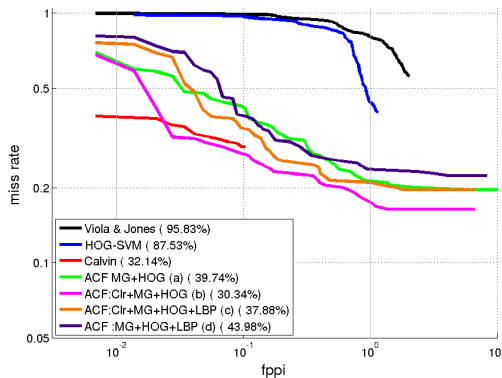
Figure 6: Log-average miss rate on InriaLite dataset.
