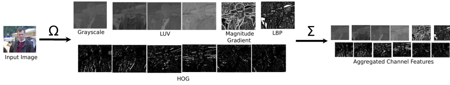
Figure 4: Aggregated Channel Features computation
