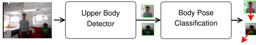
Figure 3: Adopted complete perceptual framework.
