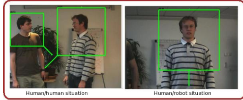
Figure 2: Output of our pose classifier in several interaction scenarios. The protruding arrows indicate pose orientation.
