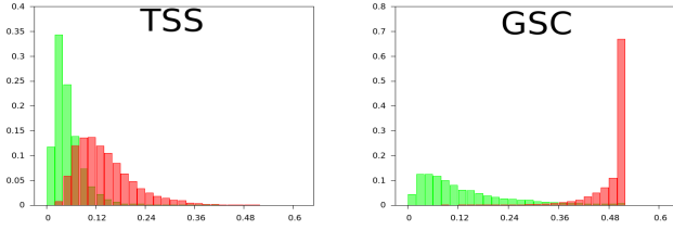
Fig. 1. Affinity costs distribution for true (in green) and false (in red) detection-track pairs on the PETS S2L2 sequence.
