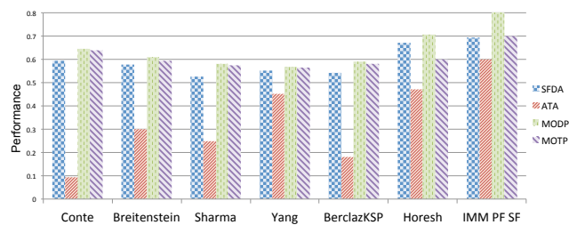
Fig. 8 Evaluation in view 1 of PETS09 S2-L1 sequence. The last diagram shows the performance of our best approach, IMM-PF SF. The others results come from [9, 17]. The results labeled Conte, Breitenstein and Shama are monocular tracking system, meanwhile Yang, BerclazKSP and Horesh are multi-view.
