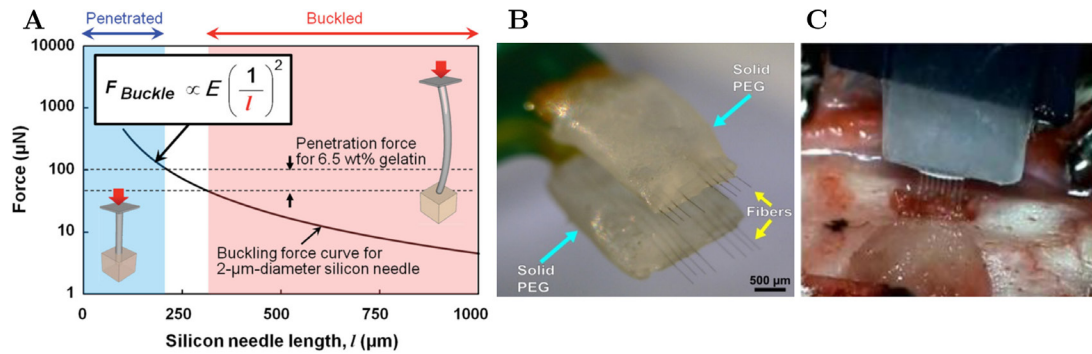
Figure 10. Reduction of effective length. (A) Buckling force versus beam length for a 2 \mu\text{m} -diameter silicon microneedle. Graph also includes an experimentally measured penetration force for gelatin (6.5 wt% in water). Therefore the blue region defines a regime where the needle will penetrate the brain, the red region where it would buckle on the surface ([179] John Wiley & Sons © 2015). (B) A carbon fiber array set in solidified PEG (light blue arrows) on both sides with submillimeter exposure of the fibers (yellow arrows) (reproduced from [180] © IOP Publishing Ltd. All rights reserved.). (C) The same technique has been applied to Parylene C shanks for insertion in rat hippocampus © (2016) IEEE. Reprinted, with permission, from [181]).
