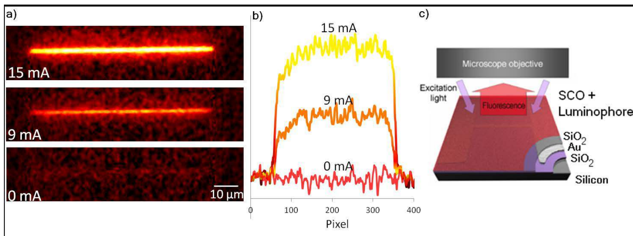
Figure 4. (a) Fluorescence microscopy images (excitation 450 nm, emission 550 nm) of a gold nanowire (80 \mu\text{m} length, 1 \mu\text{m} width, 50 nm thickness) covered by a thin film of the spin crossover compound [\text{Fe}(\text{hptrz})_3](\text{OTs})_2 doped with Rhodamine 110. During the fluorescence measurements the nanowires were heated by Joule effect: the current intensity is indicated for each image. (b) Cross-section of the fluorescence images along the nanowires. (c) Schematic picture of the device and the measurement setup.
