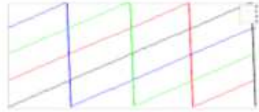
Possible shift positions of chirp for SF equal to 2
