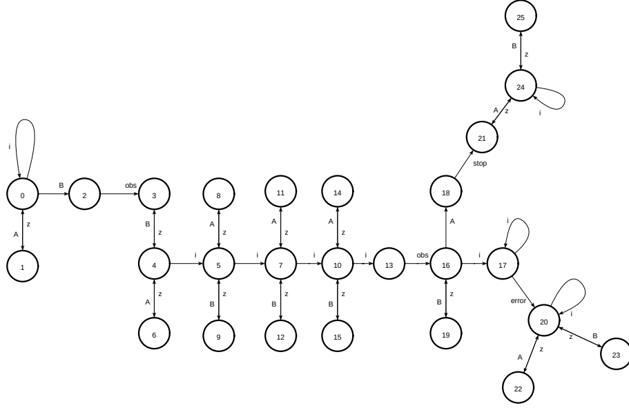
Fig. 1. State graph for the ( Universal || Present )
