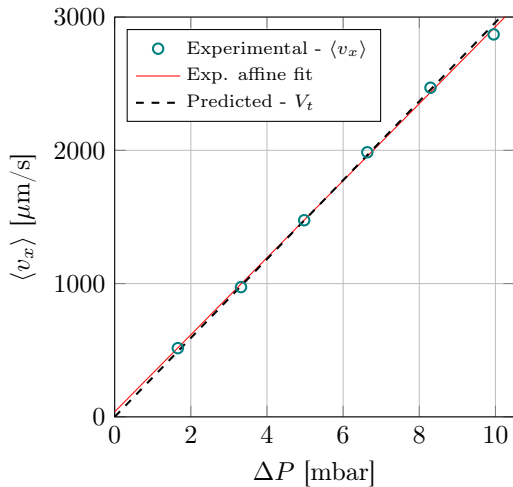
Figure 3. Experimental and predicted mean velocity of a bead ( d = 1000\text{ nm} ) flowing in a nanoslit ( h = 1300\text{ nm} ) as a function of the pressure drop. An affine fit of the experimental points is added. Error bars are smaller than the points extension.
