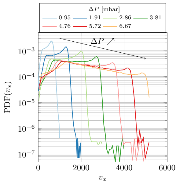
Figure 8. Probability density functions (PDF) of the longitudinal velocity v_x . Beads have a diameter d = 100 nm and are transported in nanoslits of depth h = 1650 nm. Because of lack of statistics, the case \Delta P = 7.62 mbar is not shown.
