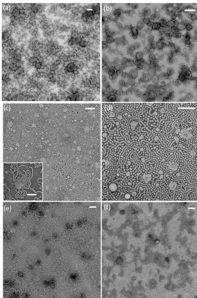
Figure 7. PEO-PBD/DPPC mixed LUV: TEM. Representative TEM micrographs of: (a) PBD-PEO and (b) DPPC nanometric vesicles; (c-f) PBD-PEO/DPPC hybrid nanometric assemblies containing (c, d) 35% DPPC and (e, f) 65% DPPC molar ratios. Scale bars of 200 nm.
