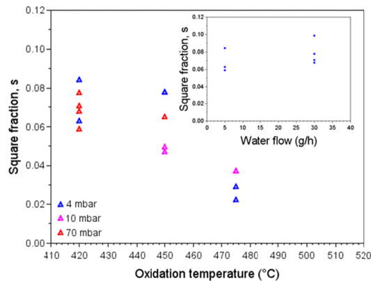
Fig. 4. Square fraction (anisotropy) of the oxide aperture (diameter around 6\mu\text{m} ) obtained from a 35\text{-}\mu\text{m} -diameter \text{Al}_{0.98}\text{Ga}_{0.02}\text{As} circular mesa versus process temperature, and (inset) versus water flow for a process temperature of 420^\circ\text{C} .
