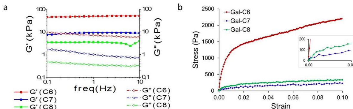
Figure 5. a. Rheology analysis of the three gels ("0-min" cooling): variation of the elastic ( G' ) and viscous ( G'' ) modulus with the frequency (strain = 2.10^{-3} (0.2%), T^{\circ}=37^{\circ}\text{C} ). b. Uniaxial compression of gels cylinders (90-min cooling; fast compression speed: 5mm/s, T^{\circ} = 20^{\circ}\text{C} , see also SI-6). Gel concentrations for both rheology and compression tests: Gal-C6: 1wt%; Gal-C7: 0.45%; Gal-C8: 0.5%.
