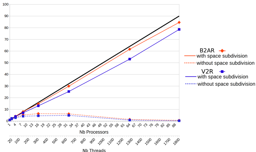
Figure 11: Evolution of the speed-up of the parallel algorithm with respect to the number of processors (working with 20 threads per processor) for the two largest molecules. Results are presented for Multi-TRRT with and without space subdivision. As a reference, the black line represents the linear speed-up.
