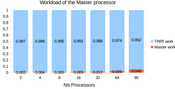
Figure 13: Proportion of the time spent by the master processor executing coordination tasks (Master work) and the exploration task (TRRT work).
