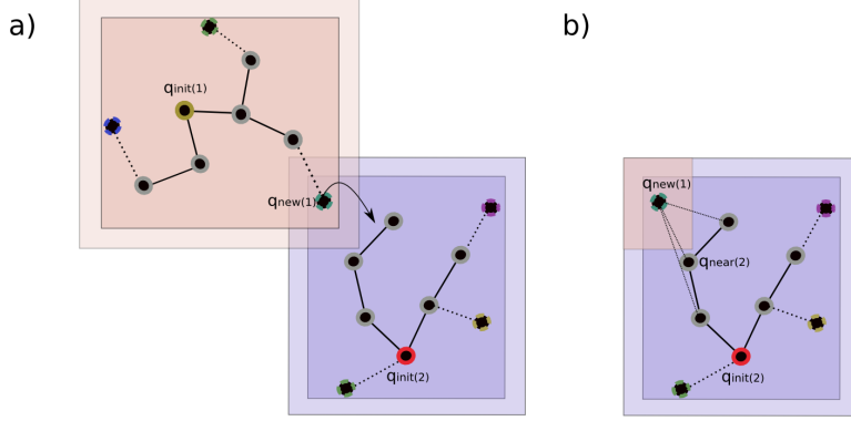
Figure 4: Illustration of the tree junction process. a) The extension of \mathcal{T}_1 generates a new node q_{\text{new}(1)} in the intersection of bounding n-polytopes \mathcal{T}_{1,2} . b) The processor in charge of the construction of \mathcal{T}_2 tries to connect q_{\text{new}(1)} to the nearest neighbor.
