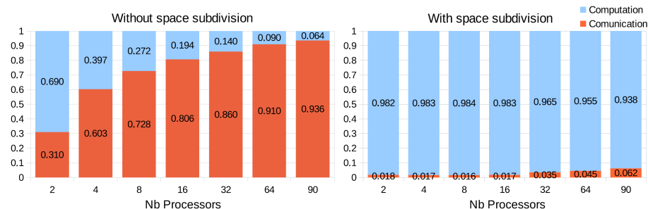
Figure 12: Proportion of the time used for computation and for communication depending on the number of processors without space subdivision (left) and with space subdivision (right).
