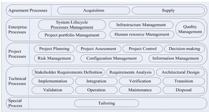
Fig. 2. Structure of the ISO/IEC-15288:2008 standard
