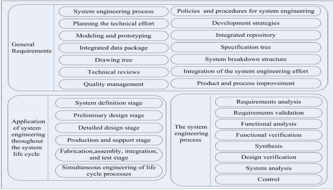
Fig. 3. Structure of the IEEE-1220:2005 standard
