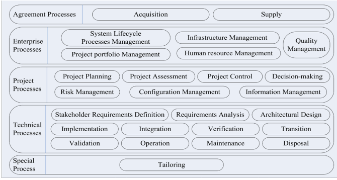
Fig. 2. Structure of the ISO/IEC-15288:2008 standard
