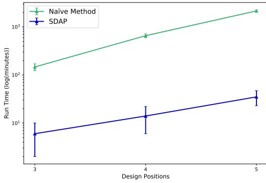
Figure 6. Evolution of the computing time (in logarithmic scale) with respect of the cardinality of the design space for the naïve approach and for SDAP.
