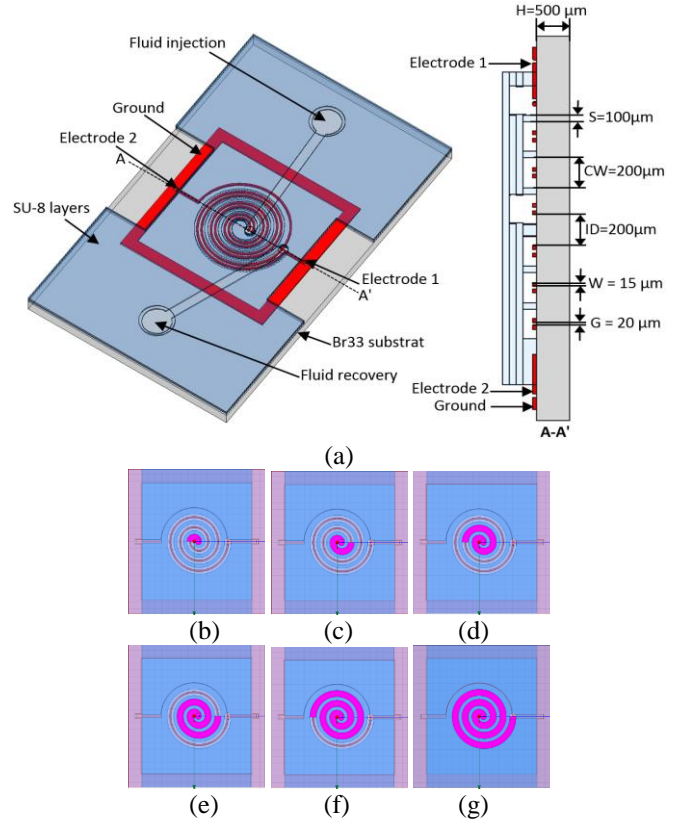
Fig. 1: (a) Tridimensional view of the microfluidic capacitor and its cross section; the six fluidic positions in the channels: (b) POS1 (c) POS 2 (d) POS3 (e) POS4 (f) POS5 (g) POS6.
