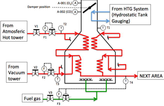
Fig. 3. Vacuum oven
