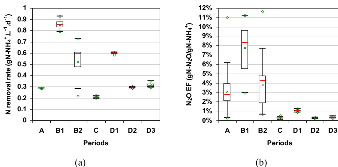
Figure 2. Statistic distributions of the evolution of the nitrogen removal rate (a) and N 2 O emission factor (b) during four different case studies. The median is represented with red thick lines, the average with green crosses, extreme values with green triangles, whiskers with vertical black lines delimited with horizontal black lines on top and bottom.
