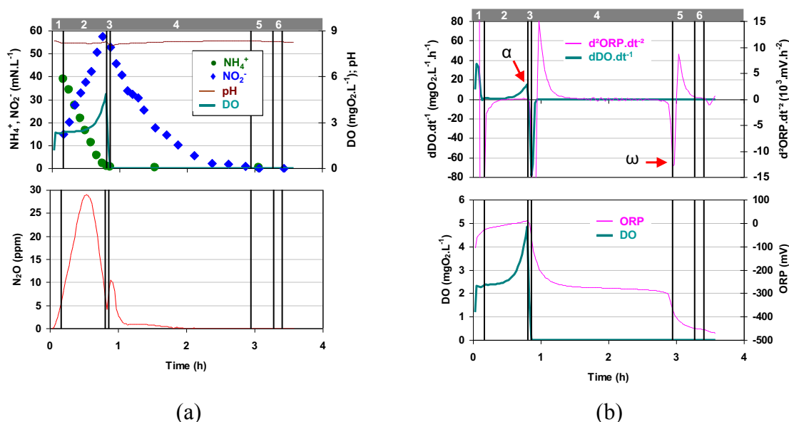
Figure 1. (a) Evolution of N-NH_4^+ , N-NO_2^- , DO, pH and N_2O during nitrification and denitrification. (b) Evolution of DO, ORP, the first derivative of DO and the second derivative of ORP during nitrification and denitrification.
