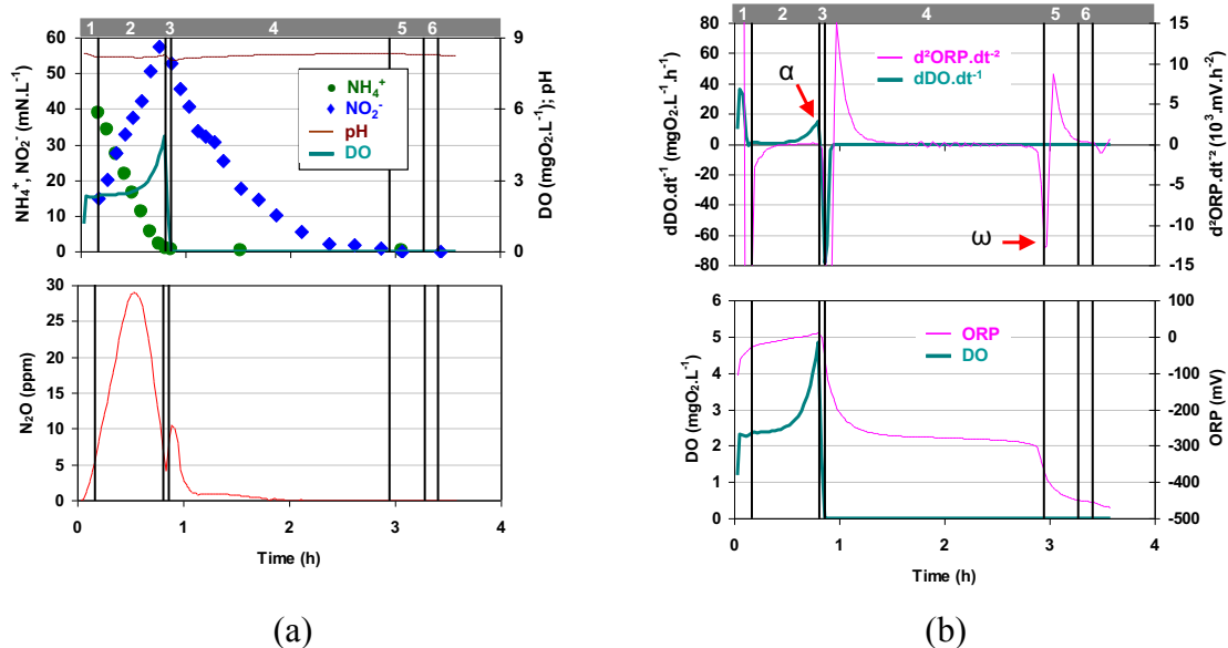
Figure 1. (a) Evolution of N-NH_4^+ , N-NO_2^- , DO, pH and N_2O during nitrification and denitrification. (b) Evolution of DO, ORP, the first derivative of DO and the second derivative of ORP during nitrification and denitrification.
