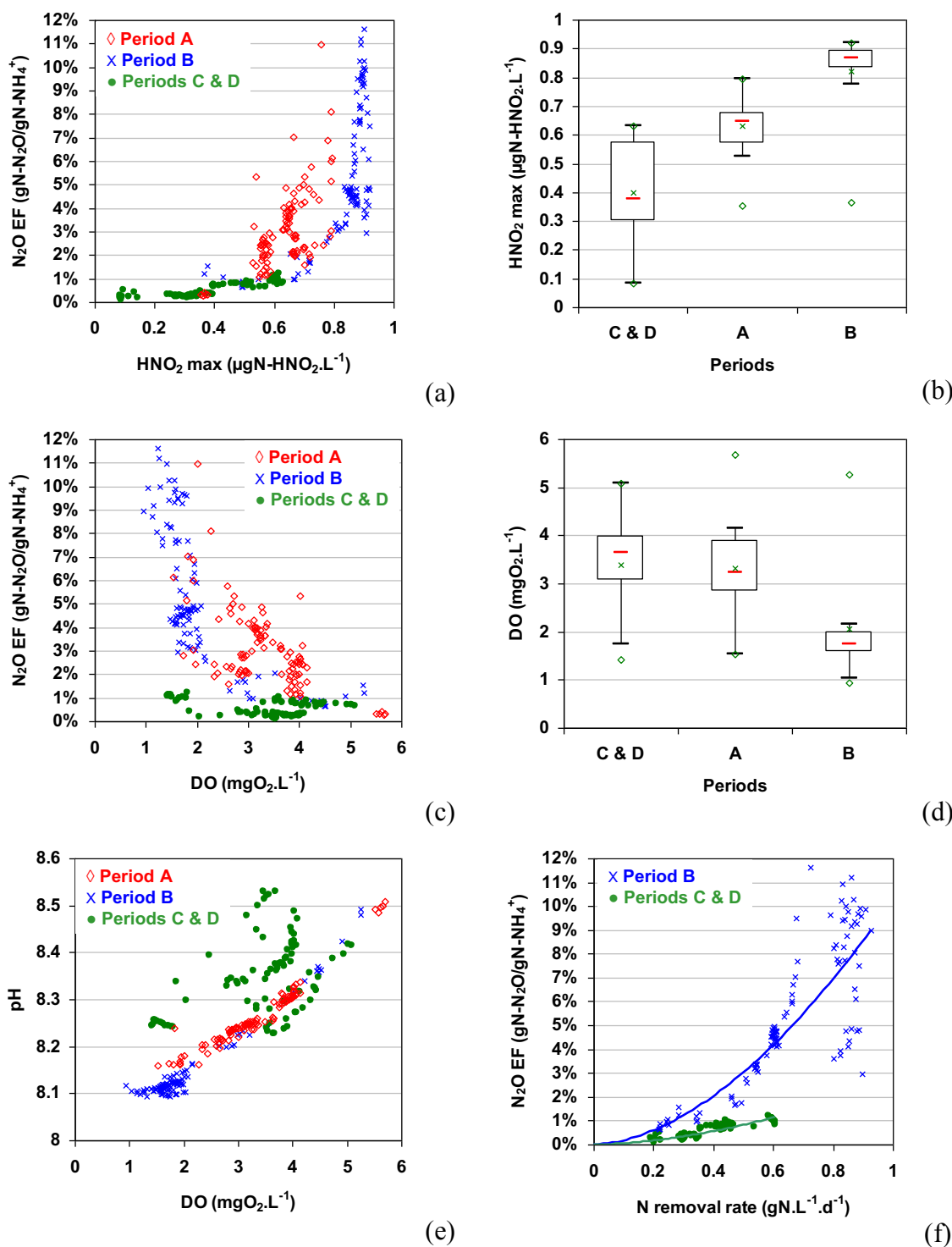
Figure 3. Maximum free nitrous acid concentration (a) and average DO during nitrification (c) versus \text{N}_2\text{O EF} for case studies A, B, C and D. Statistic distributions of the free nitrous acid concentration (b) and DO (d) during case studies. Average pH during nitrification versus DO (e) during case studies. \text{N}_2\text{O EF} versus nitrogen removal rate for case studies B, C and D (constant nitrogen removal rate with a high \text{N}_2\text{O EF} variation during phase A). Lines correspond to trend curves relative to the different data series. Each point corresponds to a SBR cycle. For statistic distributions, the median is represented with red thick lines, the average with green crosses, extreme values with green triangles, whiskers with vertical black lines delimited with horizontal black lines on top and bottom.
