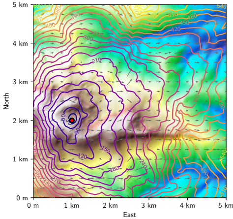
Fig. 3: Result of a fire propagation in a mountainous area. The background color indicates the heights of the digital terrain map, level curves indicate ignition times labeled in minutes relatively to the fire start, denoted as a red dot. Arrows represent the local wind speed and direction. The time required to compute this propagation is about 11s on an Intel Core i7 PC running at 2.70GHz.
