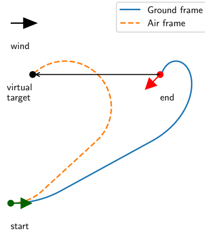
Fig. 2: Dubins trajectory under the presence of constant wind. The UAV is commanded to perform the dashed trajectory to reach the virtual target. Because of the effect of the wind, the real trajectory will be the solid line and hence attain the desired end point.
