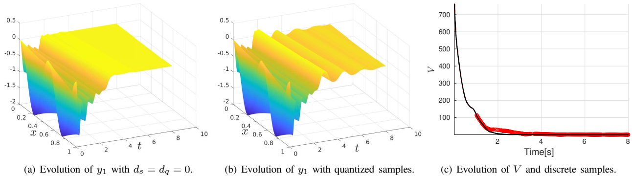
Fig. 1. Simulation results with dynamic controller.
