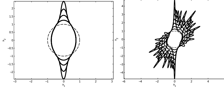
Fig. 3 Ball \mathbb{B}^2 in dashed and \cup_{k \in \mathbb{N}_i} \Omega_k , for i \in \mathbb{N}_i in solid line for Example 3, with \theta = 0 (left) and \theta = \frac{\pi}{5} (right).
