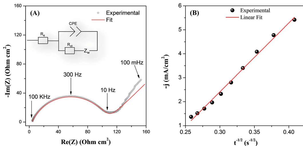
Fig. 5 (a) Nyquist plots and (b) Cottrell plot obtained for the electrophoretically deposited \text{Li}_4\text{Ti}_5\text{O}_{12} electrodes.
