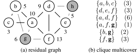
Figure 2: Explanation minimisation
