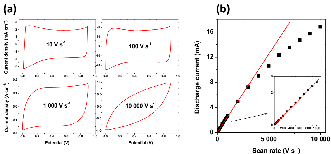
Fig. 3 Cyclic voltammetry characterizations (CV) of MWCNTs-based micro-supercapacitor. (a) CVs obtained at different scan rates in de-aerated 0.5M H 2 SO 4 electrolyte. (b) Evolution of the discharge current versus scan rate.
