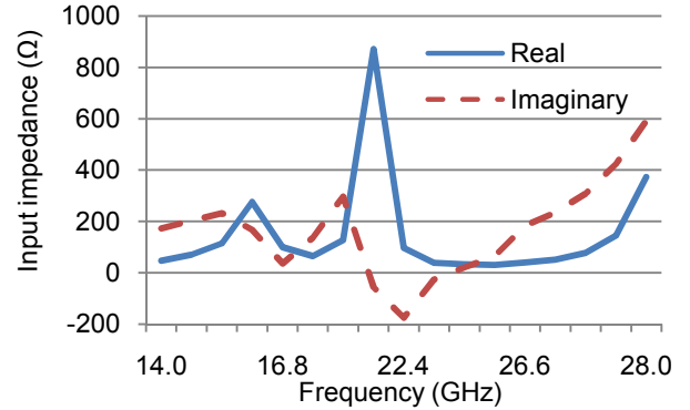
Fig. 3. Simulated (FEKO) impedance Z_{in\_a} at port p1 (see Fig. 1) when the port p2 is loaded by C=1.5\text{pF} and the port p3 is loaded by RL=250\Omega ( l_d=5.5\text{mm} and l_c=3.5\text{mm} )
