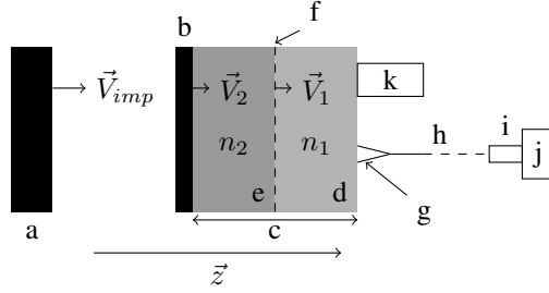
Figure 2: Sketch of the experimental setup configuration— a : Impactor, b : Aluminum coating, c : Target, d : Unshocked material, e : Shocked material, f : Shock wavefront, g : Applicator, h : Rectangular dielectric waveguide of 5 m in length, i : Rectangular metallic waveguide, j : 94 GHz source, k : Laser interferometer, \vec{V}_{imp} : Impact velocity, \vec{V}_1 : Shock wave velocity, \vec{V}_2 : Particle velocity
