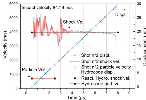
Fig. 6. Displacement, shock and particle velocity comparisons between experimental and simulation results for an impact velocity of 847.9 m/s.
