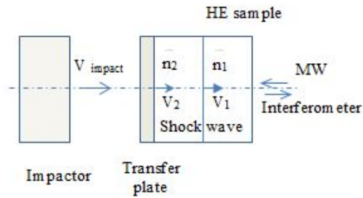
Fig. 1. Sketch of the experimental set-up.
