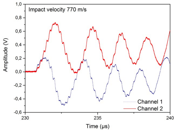
Fig. 4. Raw microwave signals for the single shock and impact velocity of 798.7 m/s.
