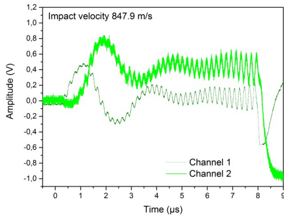
Fig. 3. Raw microwave signals for the single shock and impact velocity of 847.9 m/s.
