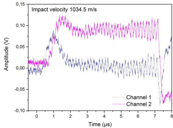
Fig. 2. Raw microwave signals for the single shock and impact velocity of 1034.5 m/s.
