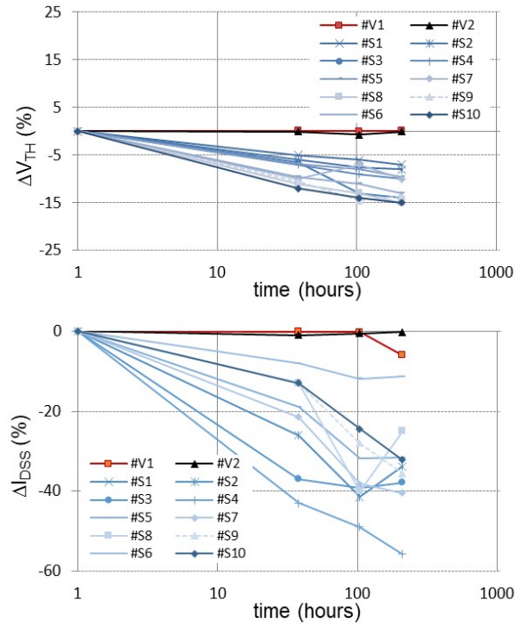
Fig. 2. Example of HTOL stress on a sample of ten 0.25 \times 8 \times 125 \mu m HEMT devices \#S_i (two virgin devices \#V_j ). Graphs report on the threshold voltage V_{TH} and on the saturation drain current I_{DSS} drifts during 210 hours of stress.
