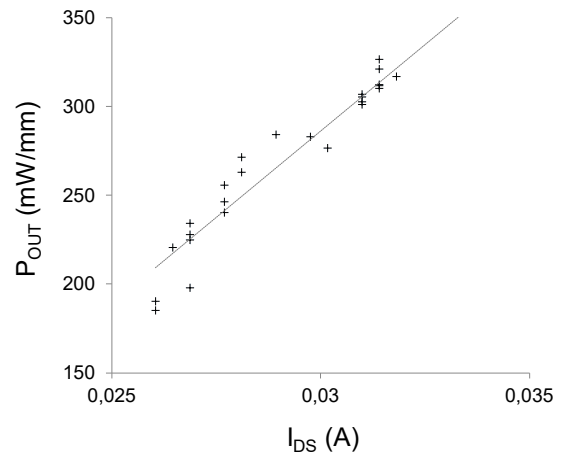
Fig. 4. Correlation between I_{DS} static current and P_{OUT} normalized output power @10GHz during 2400 hours of RF=10 GHz stress at 3dB power compression. HEMT device under test is 0.25 \times 2 \times 75 \mu m^2
