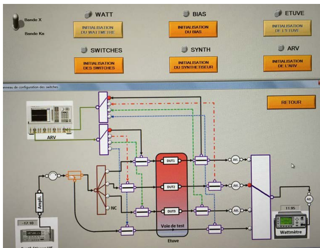
Fig. 3. Screenshot of the fully-automated workbench used for RF/thermal stresses using step stresses or CW signals ranging from 0.1 GHz to 40 GHz. Thermal cycles slopes are considered for temperature stabilization of the devices (from -40 to +150°C). Vector Network Analyser collects [S] parameters with individual calibration set for each channel at intermediate times (very small variation of the calibration during hot/cold cycles and over a large period of use, less than 0.12dB insertion losses over 2 weeks).
