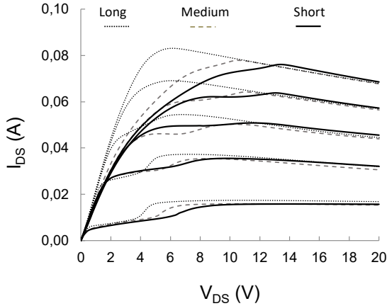
Fig. 6. Illustration of invasive DC-measurement on output characteristics of a 0.25 \times 2 \times 50 \mu\text{m}^2 HEMT (Measurement performed on a not yet mature InAlN/GaN HEMT process). I-V characteristics are given for different acquisition time configurations (acquisition time per data point - Short=640 \mu\text{s} / Medium=20ms / Long=320ms) using 4156C Keysight Signal Analyser.
