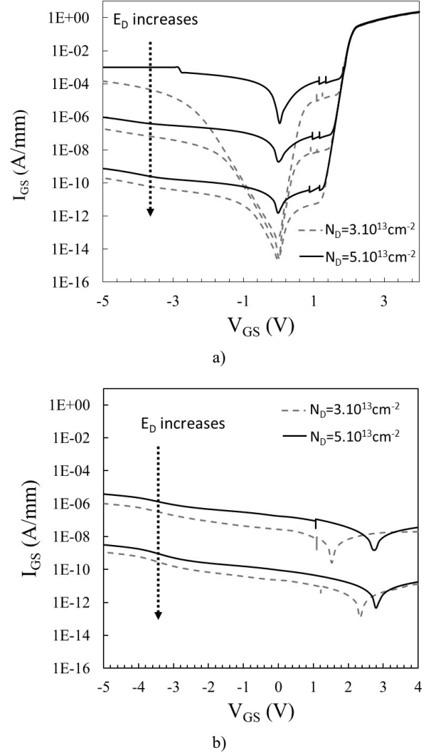
Fig. 8. Simulated leakage I_{\text{GS}}-V_{\text{GS}} characteristic ( V_{\text{DS}}=0\text{V} for figure a, and V_{\text{DS}}=8\text{V} for figure b), versus different donor activation energies and concentrations. Energies E_D are situated at (0.1eV figure a), 0.3eV and 0.5eV below the conduction band, with donor concentration n_D at 3.10^{13}\text{cm}^{-2} and 5.10^{13}\text{cm}^{-2} .
