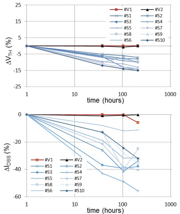
Fig. 2. Example of HTOL stress on a sample of ten 0.25 \times 8 \times 125 \mu\text{m} HEMT devices \#S_i (two virgin devices \#V_j ). Graphs report on the threshold voltage V_{TH} and on the saturation drain current I_{DSS} drifts during 210 hours of stress.
