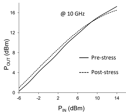
Fig. 5. P_{out} - P_{in} plot for a typical 0.25 \times 2 \times 75 \mu m^2 AlGaIn/GaN HEMT device before (line) and after (dashed) the application of RF stress for 2400 hours @ 10 GHz under 3dB compression point.
