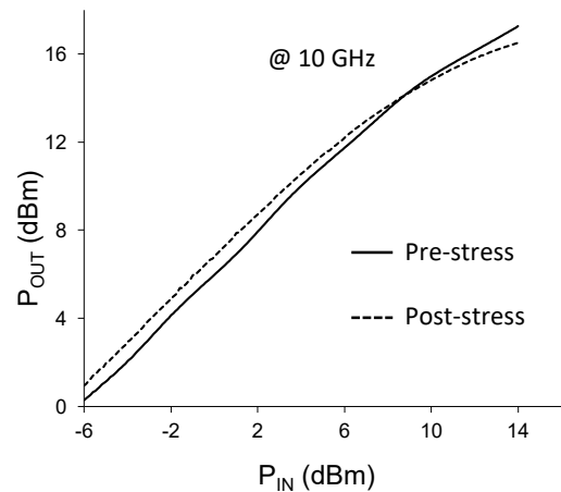
Fig. 5. P_{out} - P_{in} plot for a typical 0.25 \times 2 \times 75 \mu\text{m}^2 AlGaIn/GaN HEMT device before (line) and after (dashed) the application of RF stress for 2400 hours @ 10 GHz under 3dB compression point.
