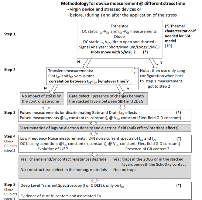
Fig. 7. Measurement methodology using transient and harmonic measurements to reveal defects in the HEMT. Comparison between initial/final measurements defines the location and the origin of the defects.
