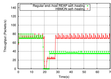
Figure 11: UDP self-healing with regular REAP and HBMON
