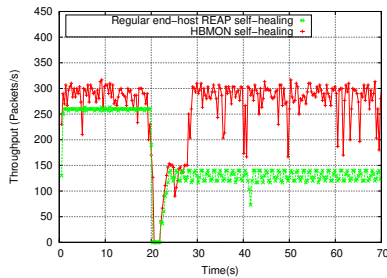
Figure 10: TCP self-healing with regular REAP and HBMON
