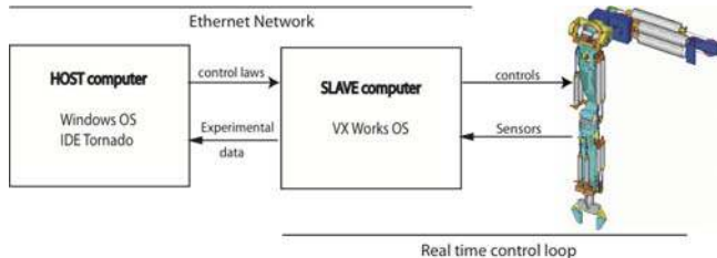
Fig. 3. Robot control architecture
