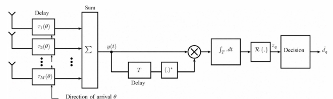
Figure 1. Multiple-antenna receiver and correlation-based detector
