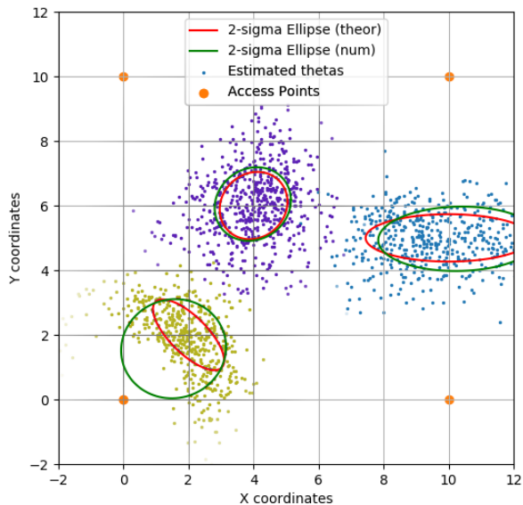
Fig. 3: A map showing the CRLB on three points with the equivalent numerically computed covariance matrix plotted in 2-sigma
