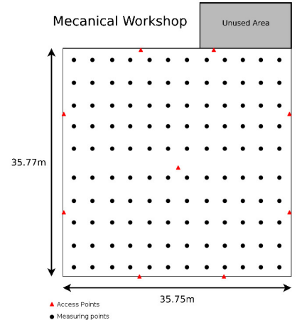
Fig. 2: Schematic of the workshop and measuring points
