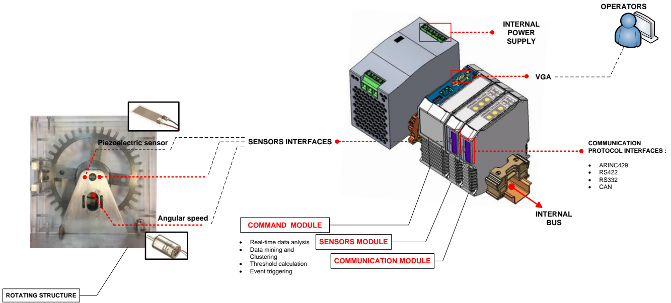
Figure 5. Experimentation setup
