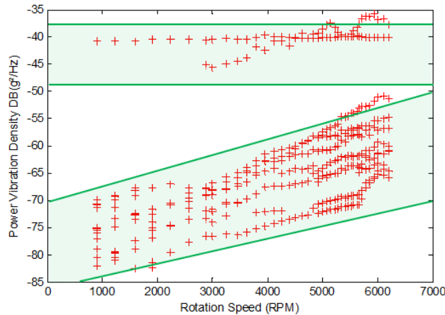
Figure 17. Abnormal signature between 700 and 6200RPM
