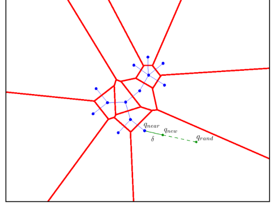
FIG. 2. RRT construction scheme. In blue/thin lines, the RRT tree. In red/bold lines, the Voronoi cells associated with the states contained in the tree. At each step, a state q_{rand} is randomly sampled, and its nearest neighbor in the search tree q_{near} is selected. It corresponds to the node in the Voronoi cell where q_{rand} has been sampled. A new node q_{new} is created by moving from q_{near} a distance \delta in the direction of q_{rand} . The Voronoi bias favors the tree expansion toward unexplored regions of the space.
