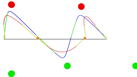
Fig. 9: Example of centroidal trajectories generated with CROC and a nonlinear solver (bird eye view), in a case of bipedal walking. The red and green circles represent the contact positions of the (respectively) left and right feet centers over time. The red and yellow (respectively related to single and double support phases) curve is the curve obtained through the concatenation of curves computed with CROC . The blue and green (respectively related to single and double support phases) curve is obtained through optimization of the latter curve with a nonlinear solver. The orange circles represent the constrained COM positions resulting from the contact planning phase, which are ignored by the nonlinear solver to produce smoother motions.
