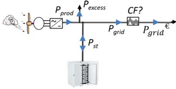
Fig. 2. Power flows.
