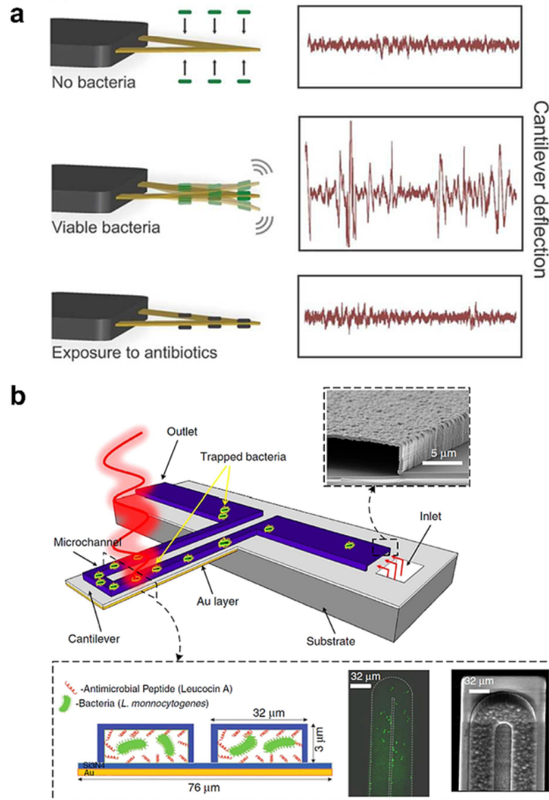
Fig. 6. High-throughput AFM-derived techniques to measure susceptibility to antimicrobial molecules. (a) Schematic description of the nanomechanical sensors developed by Kasas team. In these nanomotion susceptibility tests, when the bacteria are not attached to the sensor, the fluctuations of the AFM cantilever are driven only by thermal motion and are low. After the attachment of live bacteria, the fluctuations are linked to their metabolic activity and are high. Finally, after exposure to a bactericidal drug, the bacteria are non-viable and the fluctuations return to low levels. (b) Schematic representation of microfluidic biomaterial cantilevers (BMC) developed by Etayash et al. The BMC is filled with bacteria supported on a silicon substrate. At the bottom, it is coated with a 300 nm-thick layer of gold, which serves as a second element. The BMC is coated with a bacteria-targeted receptor and irradiated with a specific wavelength of tunable infrared light. The inset on top is a SEM image of the cross-section of an inlet, located on bottom side of the chip. An aqueous solution of bacteria is loaded from the inlet. In the lower panel, a cross-section of the 32 mm wide microchannel of the cantilever is presented. On the right is presented a fluorescent image from the top side of the BMC, filled with bacteria, and a SEM image of the tip of the BMC. When the bacteria inside the BMC absorb infrared light, local heat is generated that results in the nanomechanical deflection of the BMC. The resonance frequency is sensitive to the increased mass caused by the adsorption of bacteria inside the BMC. When the BMC is illuminated with a certain range of infrared light, a plot of the nanomechanical deflection of the BMC shows the wavelength where the bacteria absorb infrared light. This can provide excell.
