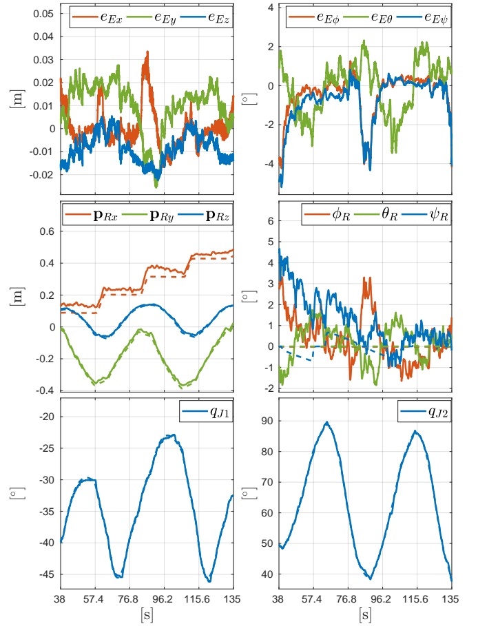
Fig. 8: Main variables when the aerial manipulator subjected by an external force produce by wind.
