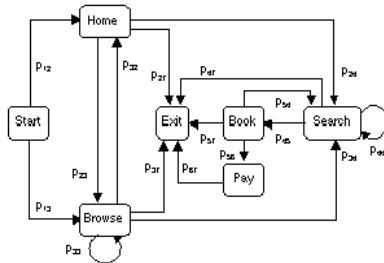
Figure 2. User operational profile graph
