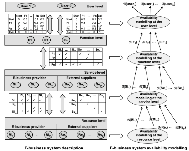
Figure 1. Hierarchical availability modeling framework
