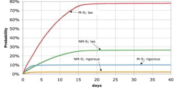
FIGURE 16. Evolution of PC(t) in M-S compared with NM-S
