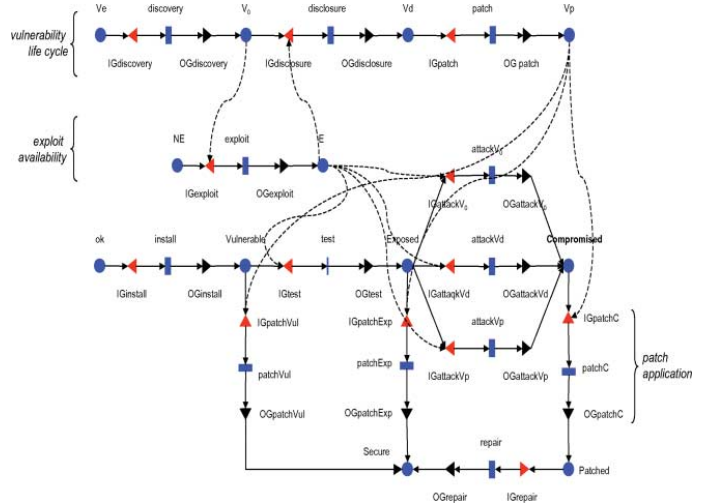
Figure 4. Vulnerability exploitation process model: M-S
