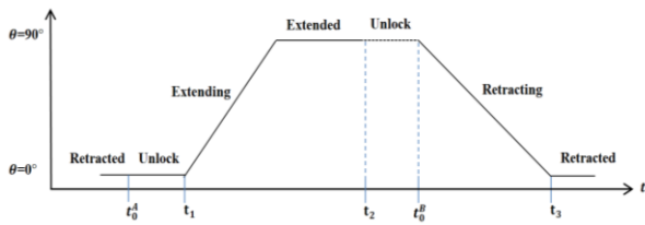
Figure 6: Landing gear output requirement
